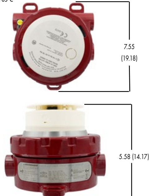
Figure 2—U5015 Dimensions in Inches (cm)
