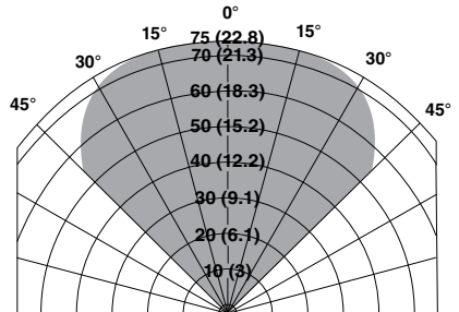
Field of View at Indicated Distance in Feet (m) for Propane at Medium Sensitivity (32-inch plume)
