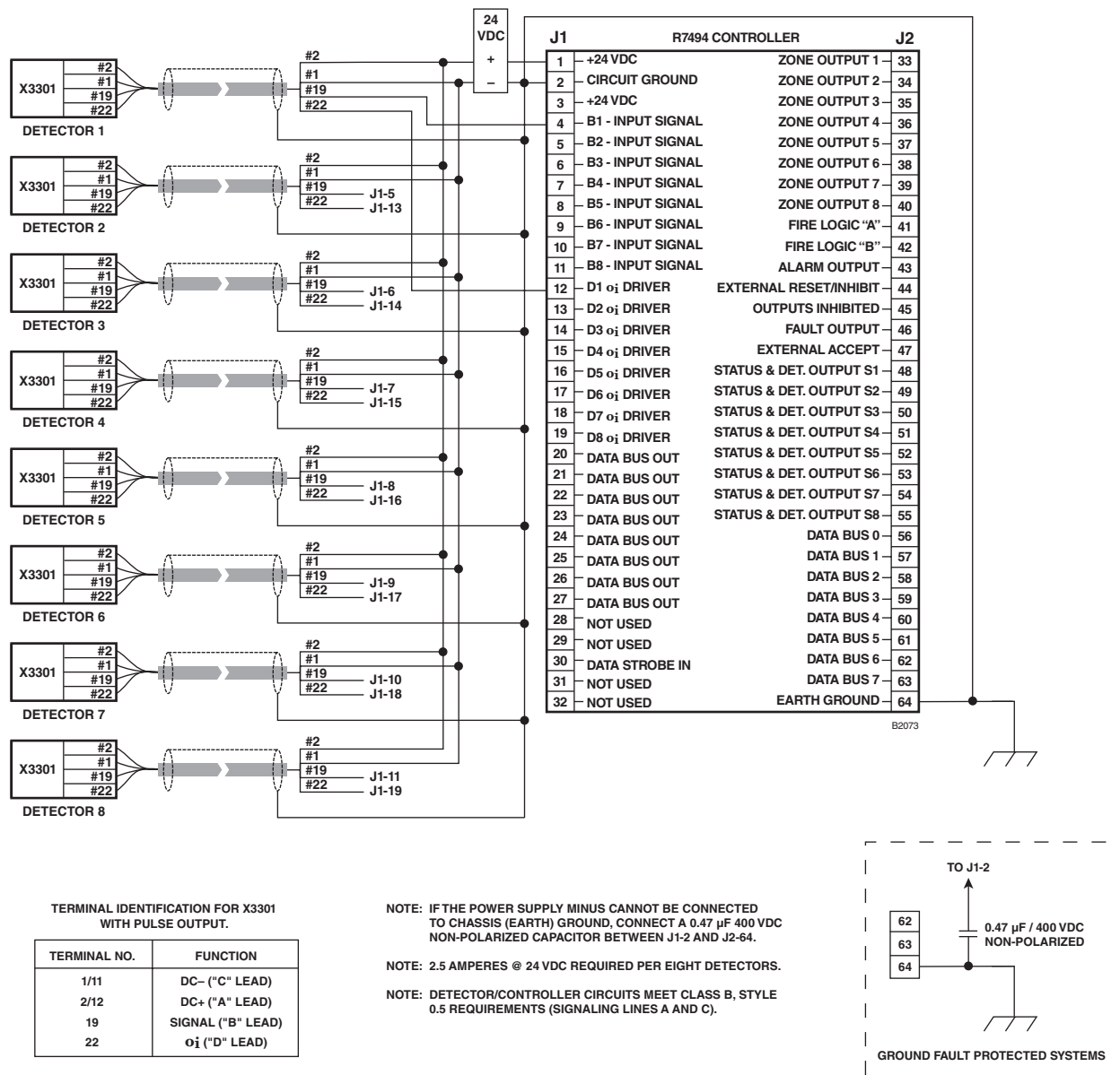
Figure 8—A Typical System, X3301 Detectors Wired to R7494 Controller
