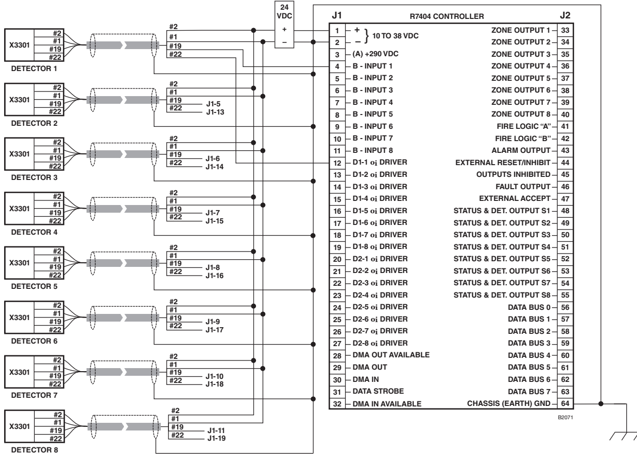
TERMINAL IDENTIFICATION FOR X3301 WITH PULSE OUTPUT.
