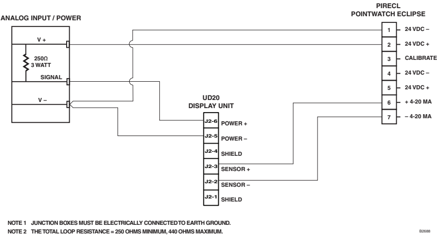
Figure 20—PIRECL Detector Wired to UD20 (Non-Isolated 4-20 mA Output, Sinking, 4-Wire)
