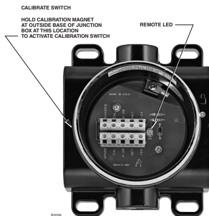
Figure 17—Remote Calibration Switch and LED in Optional Det-Tronics PIRTB Termination Box
