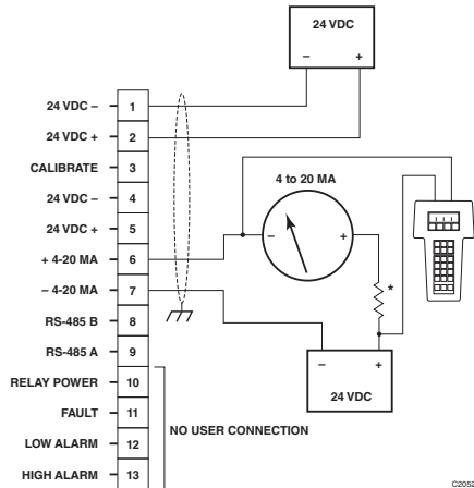
Figure 10—Eclipse Detector Wired for Isolated 4-20 mA Current Output (Sinking)
