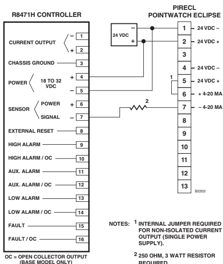
Figure 14—Standard Eclipse Wired to a Model R8471H Controller
