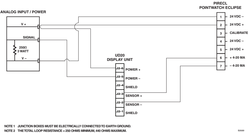
Figure 21—PIRECL Detector Wired to UD20 (Non-Isolated 4-20 mA Output, Sourcing, 4-Wire)
