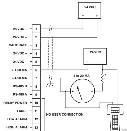
Figure 11—Eclipse Detector Wired for Isolated 4-20 mA Current Output (Sourcing)
