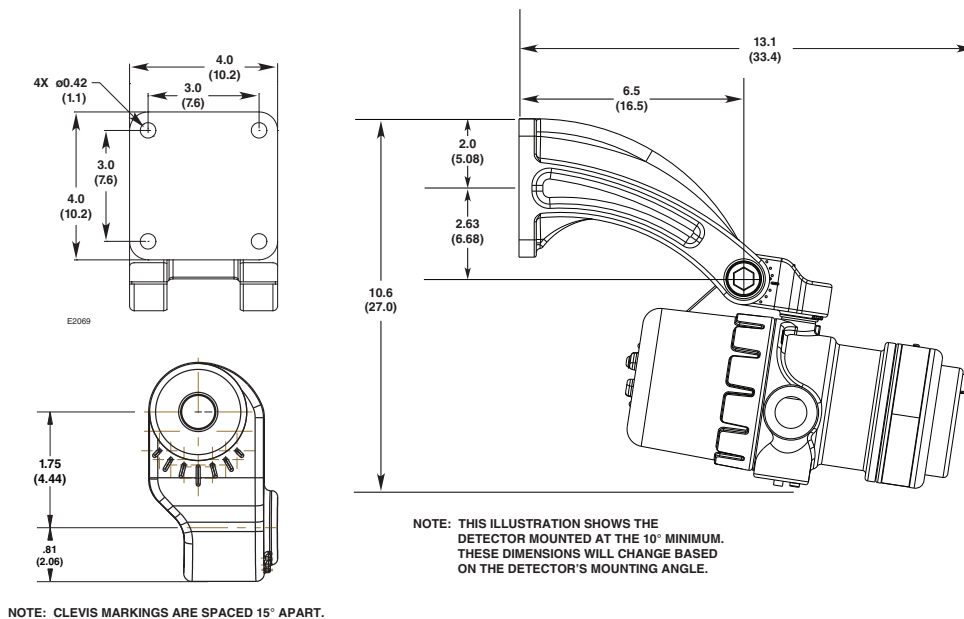
Figure 2—Q9033 Mounting Arm Dimensions in Inches (cm)
