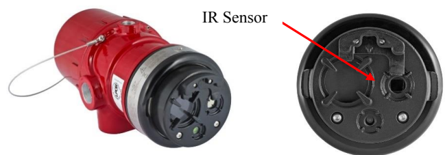
Figure 6: Det-Tronics X9800 IR technology optical flame detector
