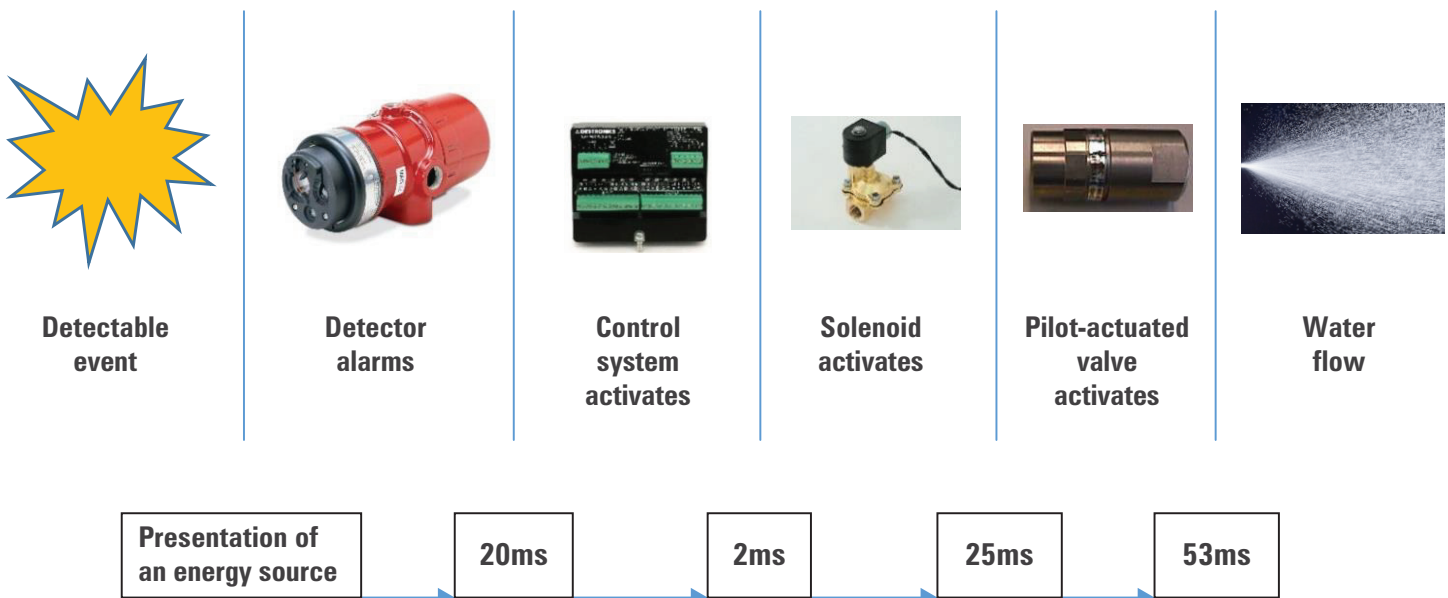
Figure 12: Response time for an entire ultra-high-speed detection and suppression system from presentation of an energy source at the detector to flow of water from the water spray nozzle cannot exceed 100 milliseconds (ms).
