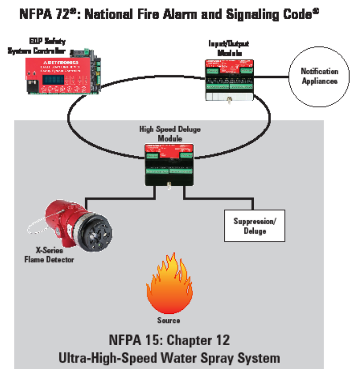
Figure 11: Visual depiction of an ultra-high-speed capable Det-Tronics system
