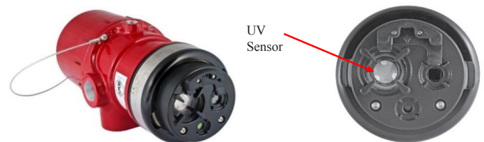
Figure 3: Det-Tronics X2200 UV technology optical flame detector
