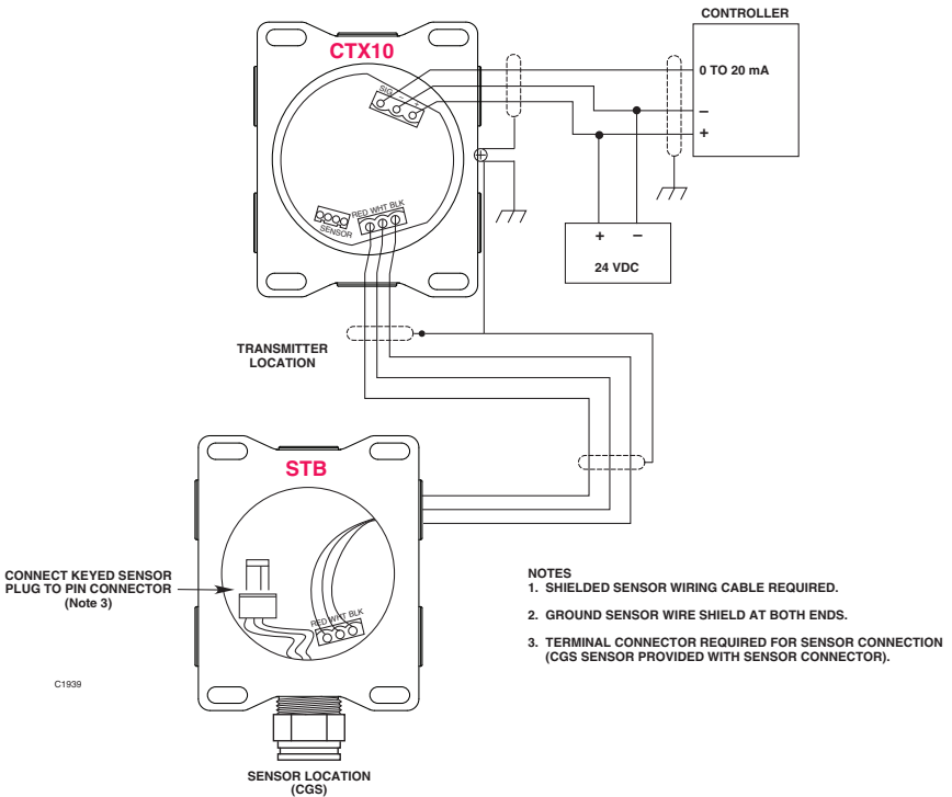
Figure 4—CGS direct mounted to STB which is connected to CTX10
