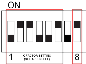
Figure B: Switch Settings for CTX10 in 505, Ininiti Mode(s)
