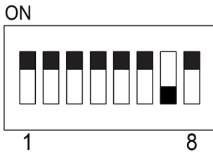
Figure C: Switch Settings for CTX10 in UD10/UD30 Mode
