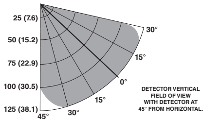
Field of View at Indicated Distance in Feet (m) for Hydrogen at Very High Sensitivity (30 inch plume, with 100 SLPM flow rate)
