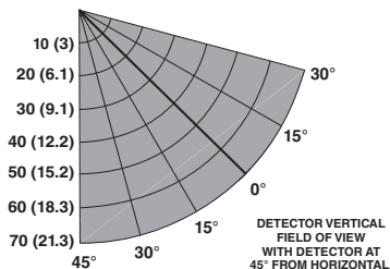
Field of View at Indicated Distance in Feet (m) for Methanol at Very High Sensitivity (1 x 1 ft)
