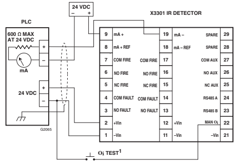
Figure 12—X3301 Detector Wired for Isolated 0 to 20 mA Current Output (Sourcing)
