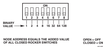
Figure 18—Address Switches for X3301 A2190
