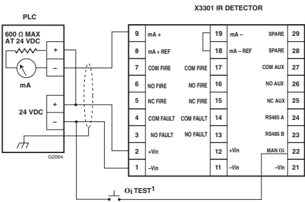
Figure 11—X3301 Detector Wired for Non-Isolated 0 to 20 mA Current Output (Sinking)
