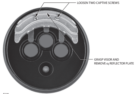
Figure 19— o i Reflector Plate Removal
