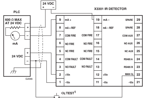
Figure 13—X3301 Detector Wired for Isolated 0 to 20 mA Current Output (Sinking)
