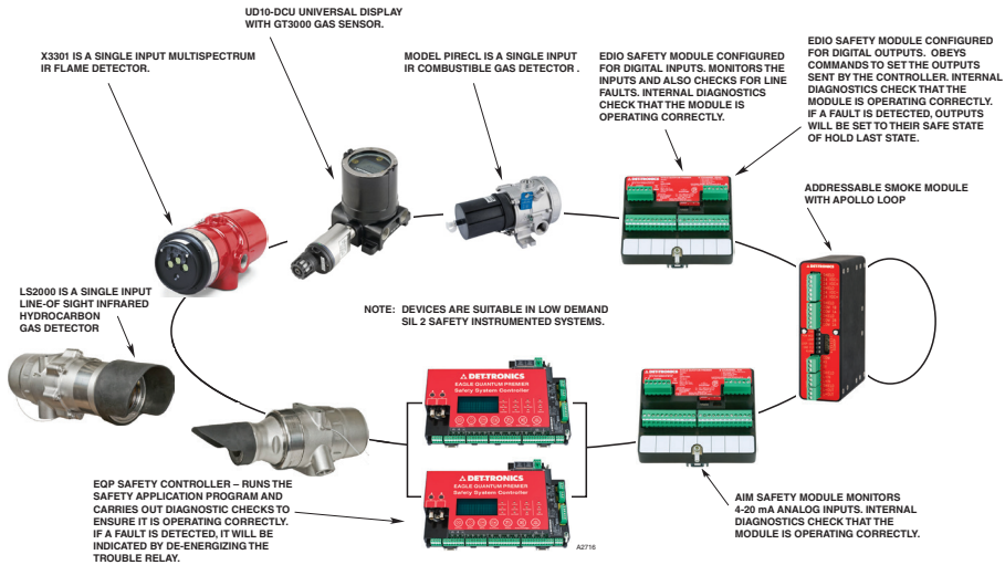
Figure 2—Det-Tronics EQP Safety System Component Overview
