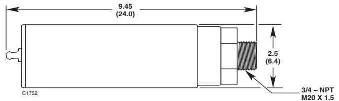
Figure 1—Aluminum PointWatch Unit Dimensions in Inches (cm)
