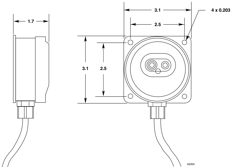
Figure 1—Dimensions of PM-5MPX in Inches
