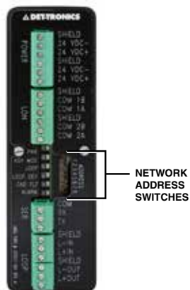
Figure 8—Location of Network Address Switches
