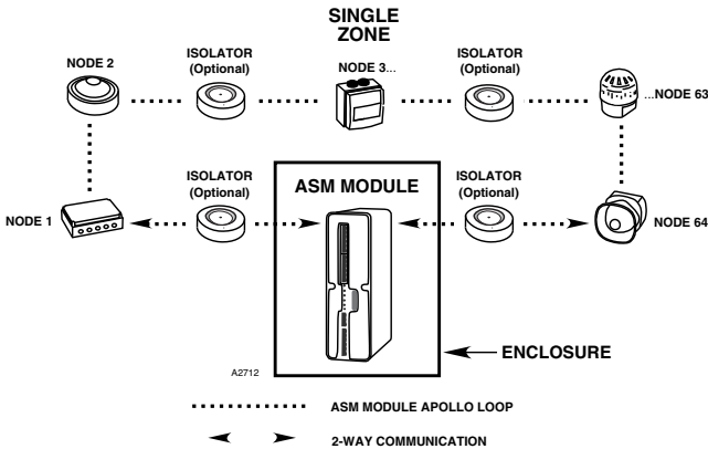
Figure 3—Class A Pathway (isolators are optional)
