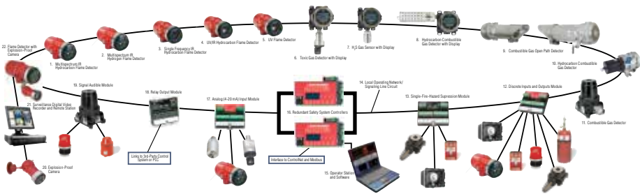
Figure 1—Components of a Det-Tronics EQP System
