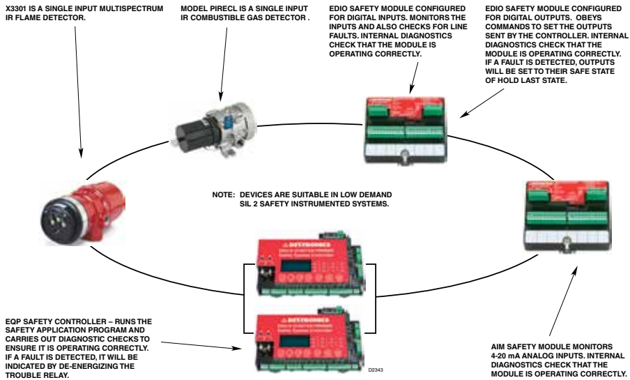
Figure 2—Det-Tronics EQP Safety System Component Overview
