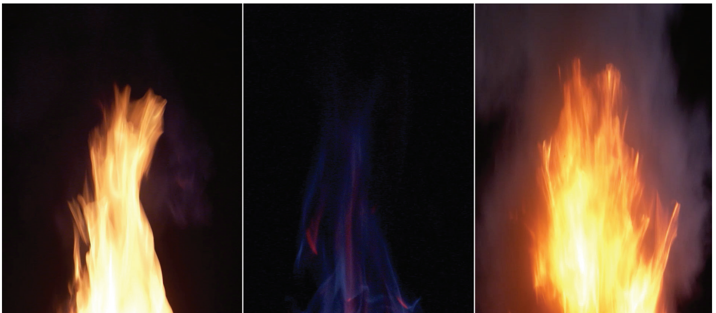
Figure 2: Every combustible gas burns differently, producing a signature flame. Compared to hydrocarbon flames depicted on the right and left above, a hydrogen flame (center) emits little visible light and IR radiant heat and therefore is more difficult for people and equipment to detect.
