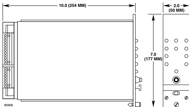
Figure 6—R7495 Controller Dimensions in Inches (MM)
