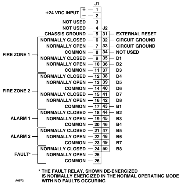
Figure 19—Terminal Configuration
