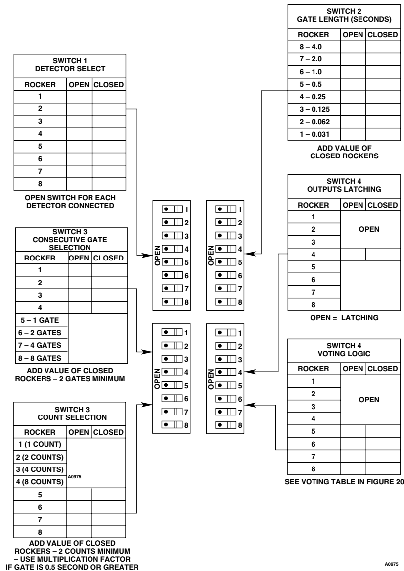
Figure 23—System Layout Chart
