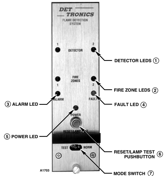
Figure 3—R7495B Controller Front Panel
