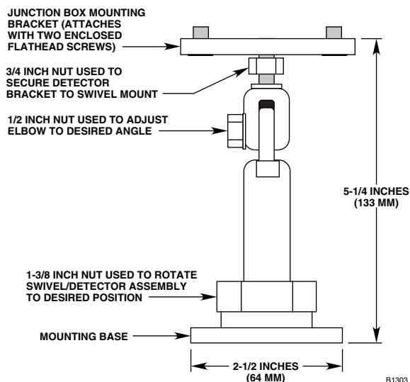
Figure 8—Q9001G Swivel Mounting Bracket Dimensions
