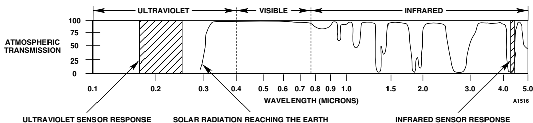
Figure 1—Detector Sensitivity Range
