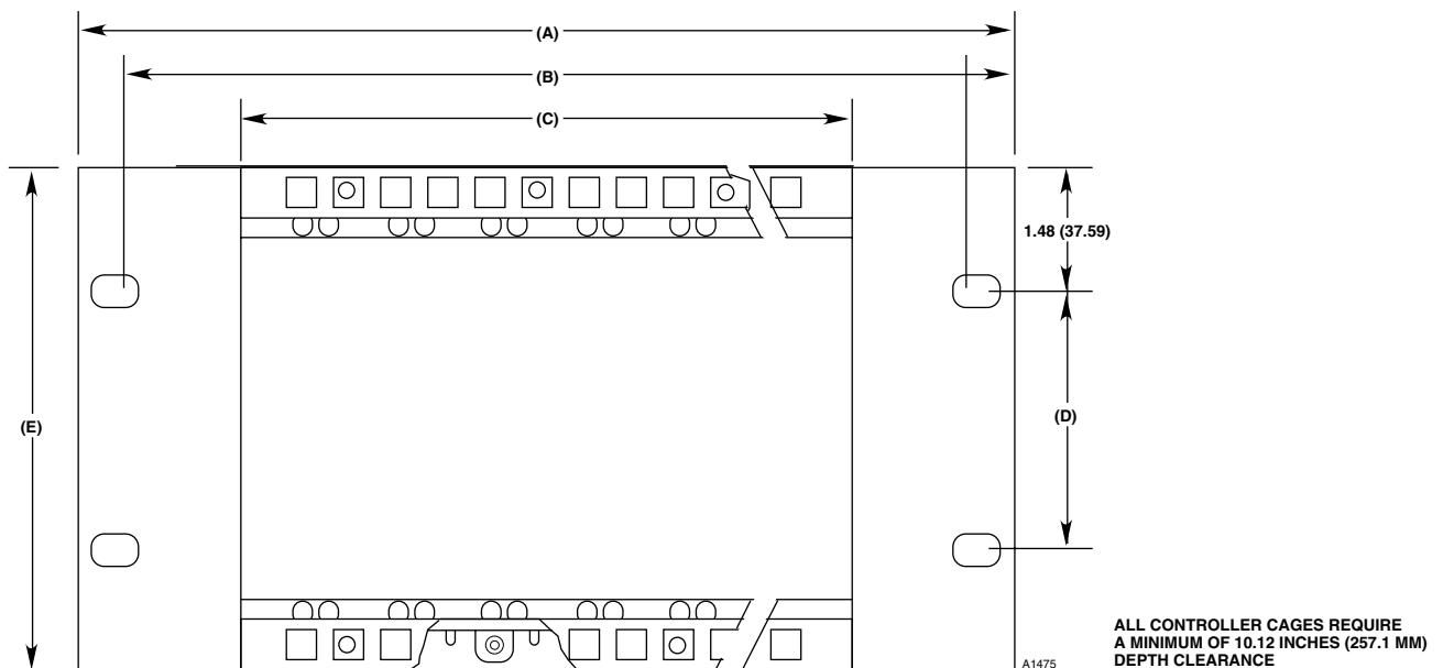
Figure 18—Q4004 Mounting Cage Dimensions in Inches (MM)
