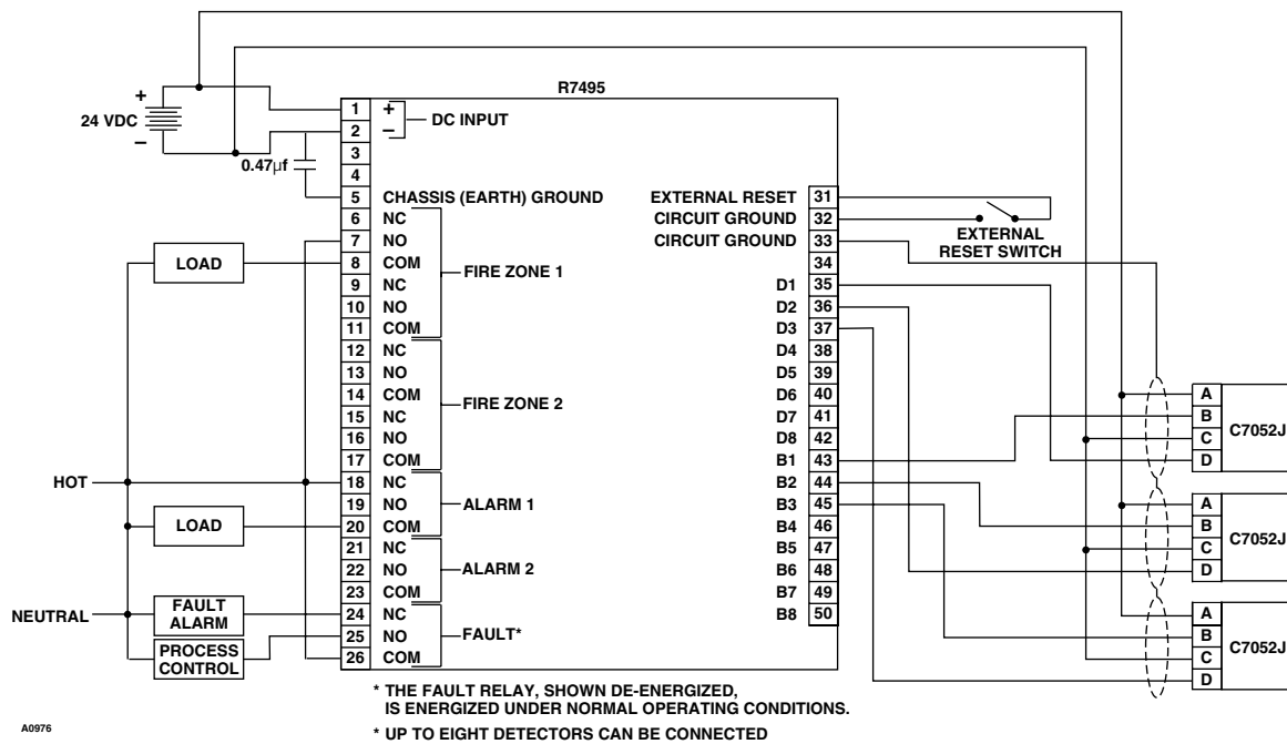
Figure 14—Typical Application Wiring
