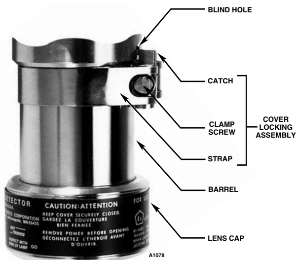
Figure 15—Cover Locking Assembly (Optional)
