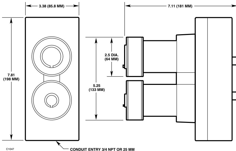
Figure 5—Detector Dimensions in Inches (MM)
