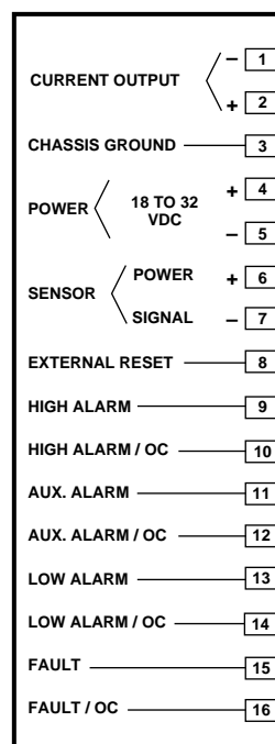
OC = OPEN COLLECTOR OUTPUT (BASE MODEL ONLY) B1390
